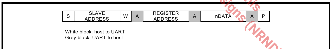
FIGURE 4. MASTER WRITES TO SLAVE (XR20M1170)
