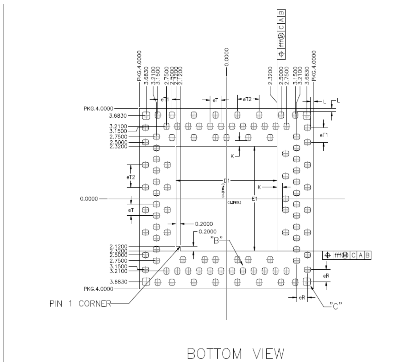
Figure 62 LGA 8 mm x 8 mm Package Outline
