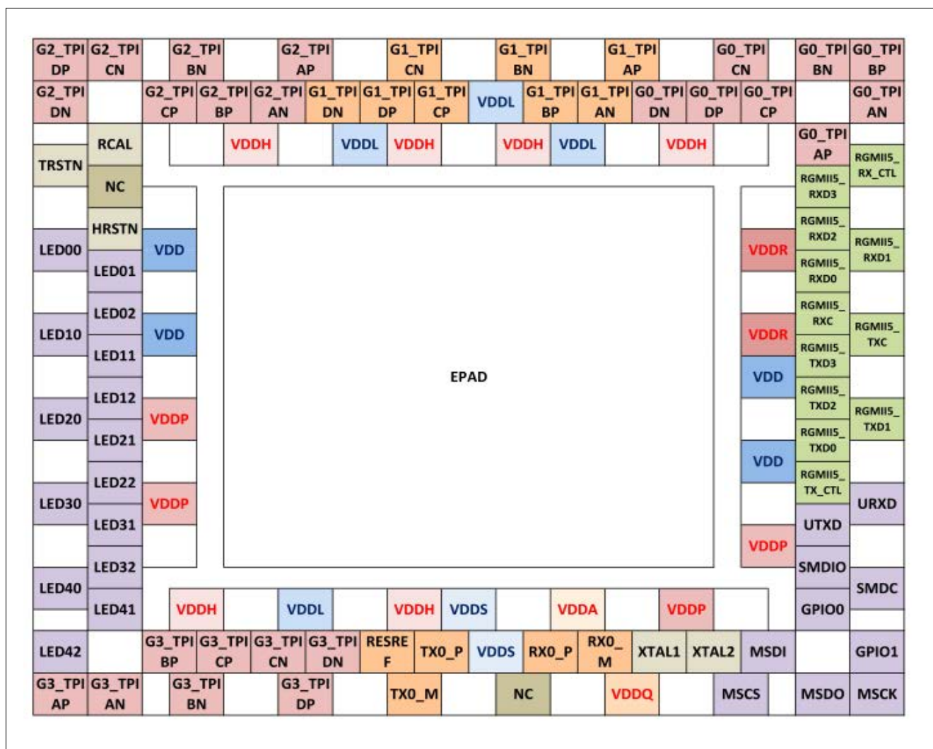
Figure 6 Pin Layout
