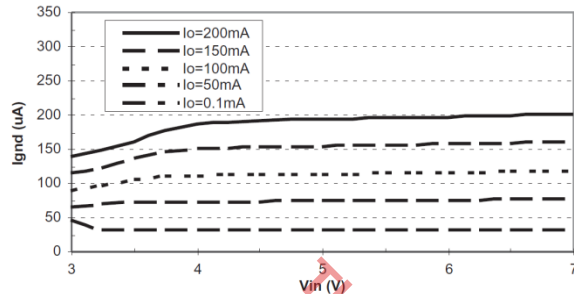
Fig. 10: I_{GND} vs. V_{IN} (SP6201 fixed 3.0V)
