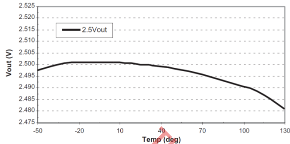
Fig. 16: V_{OUT} vs. Temp (adjustable)
