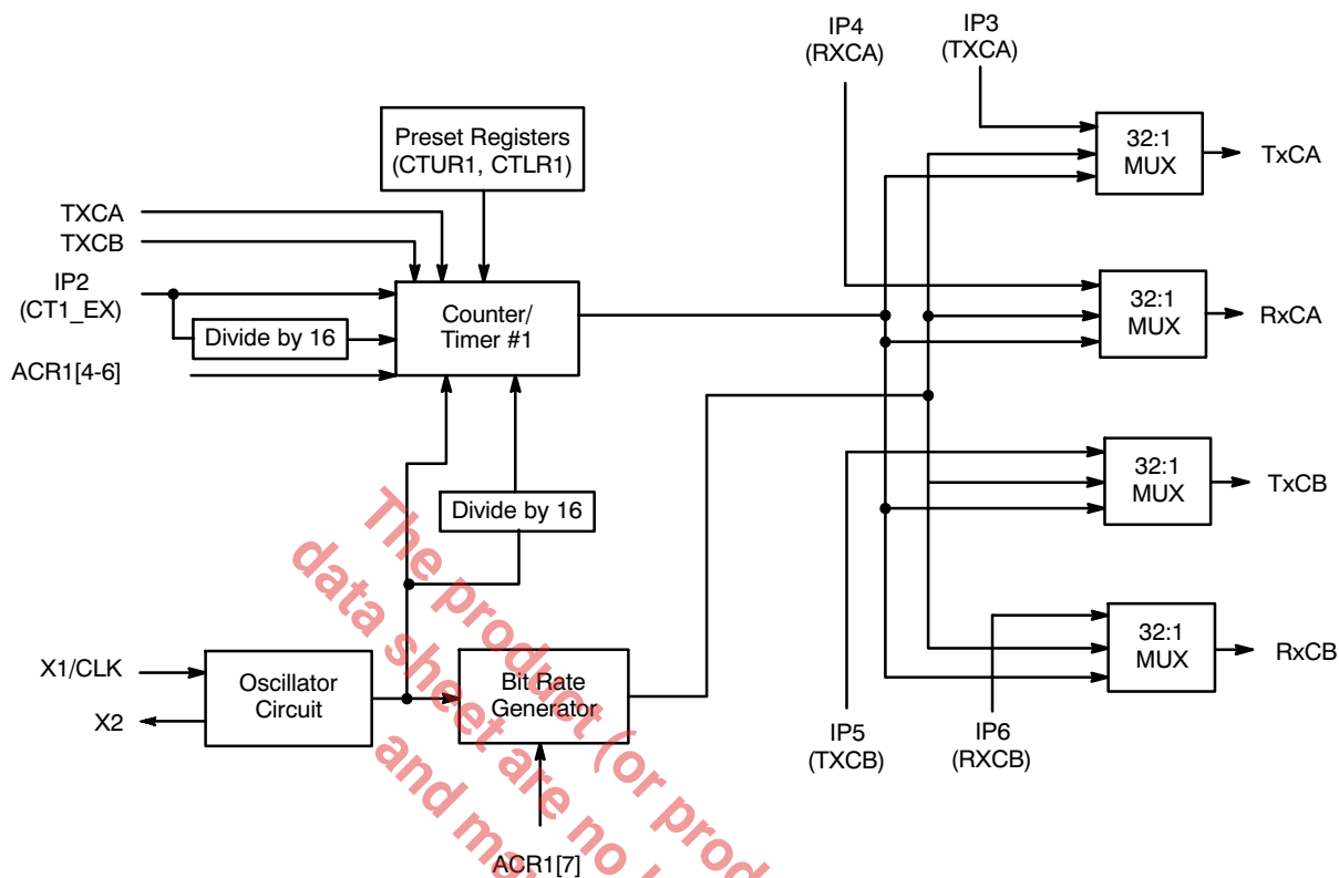
Figure 28. Block Diagram of the Portion of the QUART Timing Control Block Which Services Channels A and B
