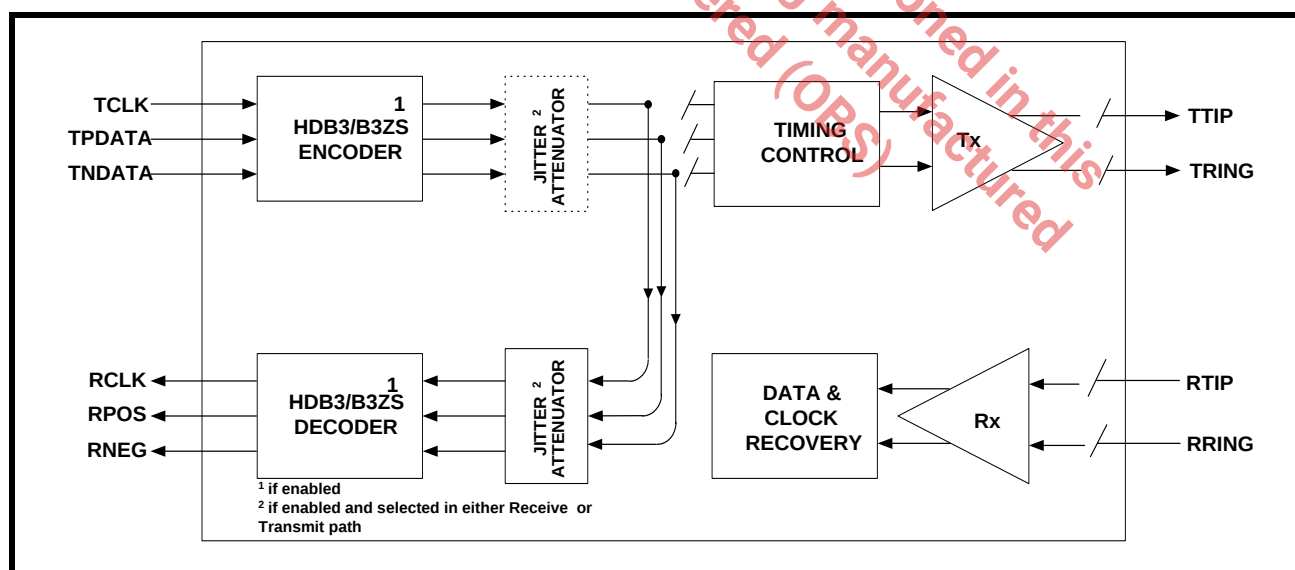
FIGURE 27. DIGITAL LOOPBACK
