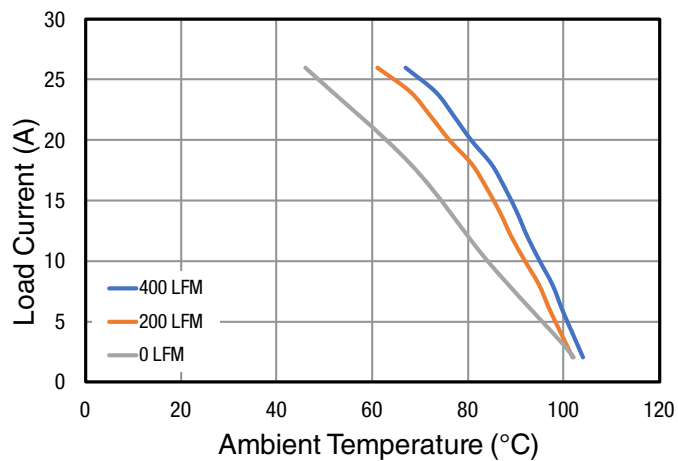
Figure 39: Current Derating, V_{IN} = 12V , V_{OUT} = 5V
