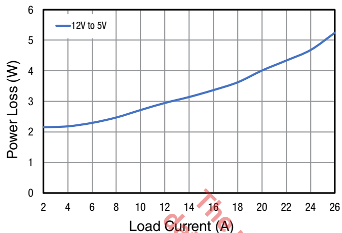
Figure 38: Power Loss, V_{OUT} = 5V
