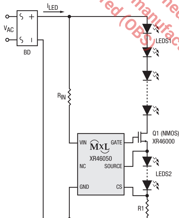
Figure 1. Typical Application
