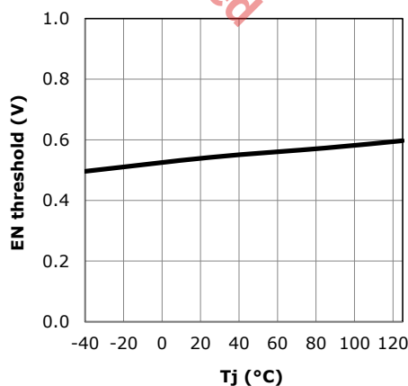
Fig. 8: Enable threshold versus temperature
