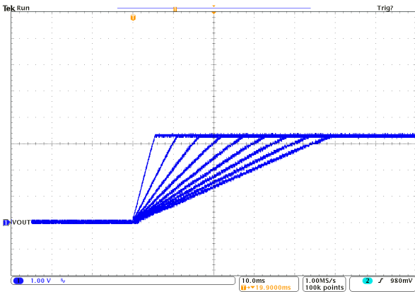
Figure 9: Simultaneous Start-Up
