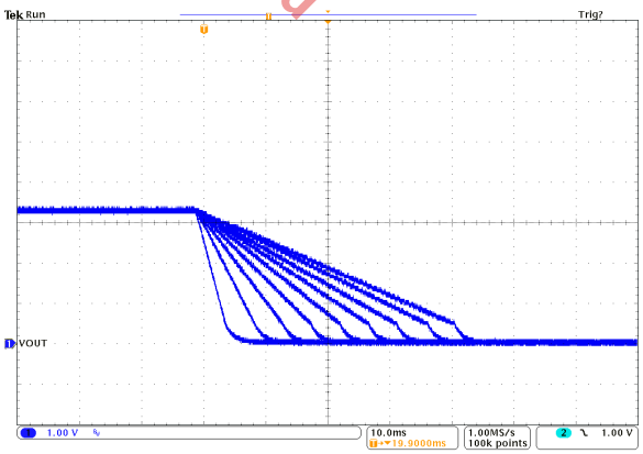
Figure 10: Simultaneous Shut-Down
