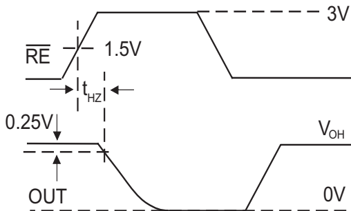
Receiver Enable and Disable Timing Diagram
