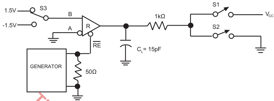
Receiver Enable and Disable Times Test Circuit
