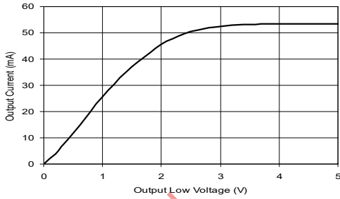
Output Current vs Receiver Output Low Voltage
