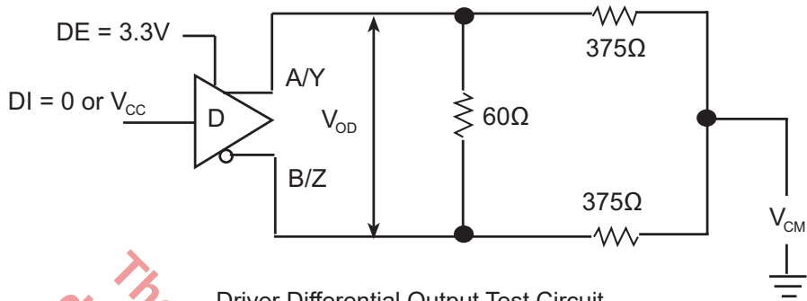
Driver Differential Output Test Circuit
