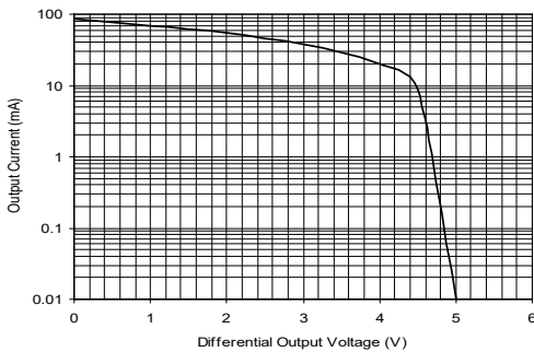
Driver Output Current vs Differential Output Voltage
