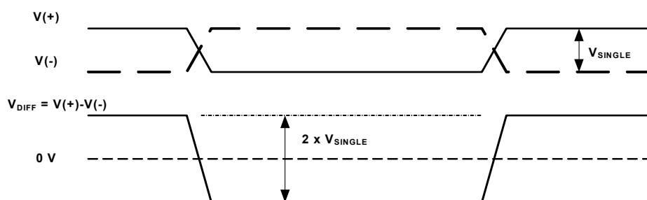
FIGURE 28. DIFFERENTIAL VOLTAGE SWING DEFINITIONS (INPUT OR OUTPUT) FOR CLOCK AND DATA
