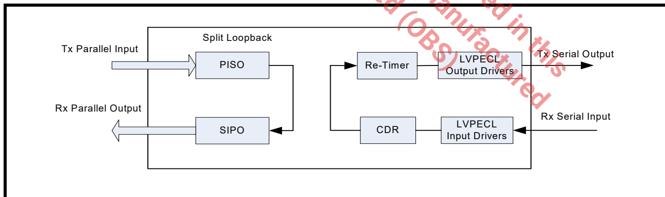
FIGURE 21. SPLIT LOOPBACK
